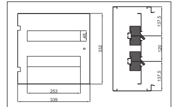
Enclosure W400 x H400 mm Product Code: 943.857
