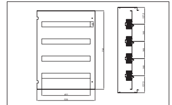
Enclosure W600 x H800 mm Product Code: 943.862
